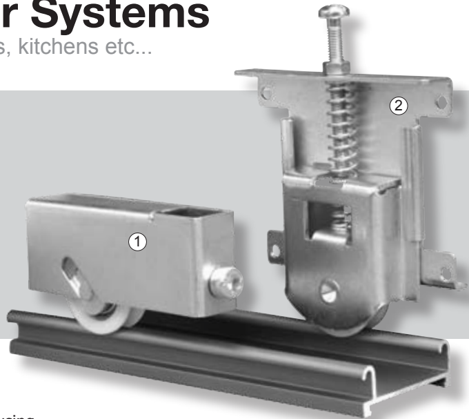
① Concealed hardware ② Adjustable hardware
