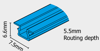
LA04530A Aluminium upper / lower guide rail
