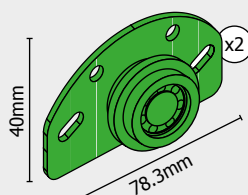
LA008811 Lower hardware
