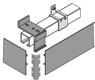
cover rail
